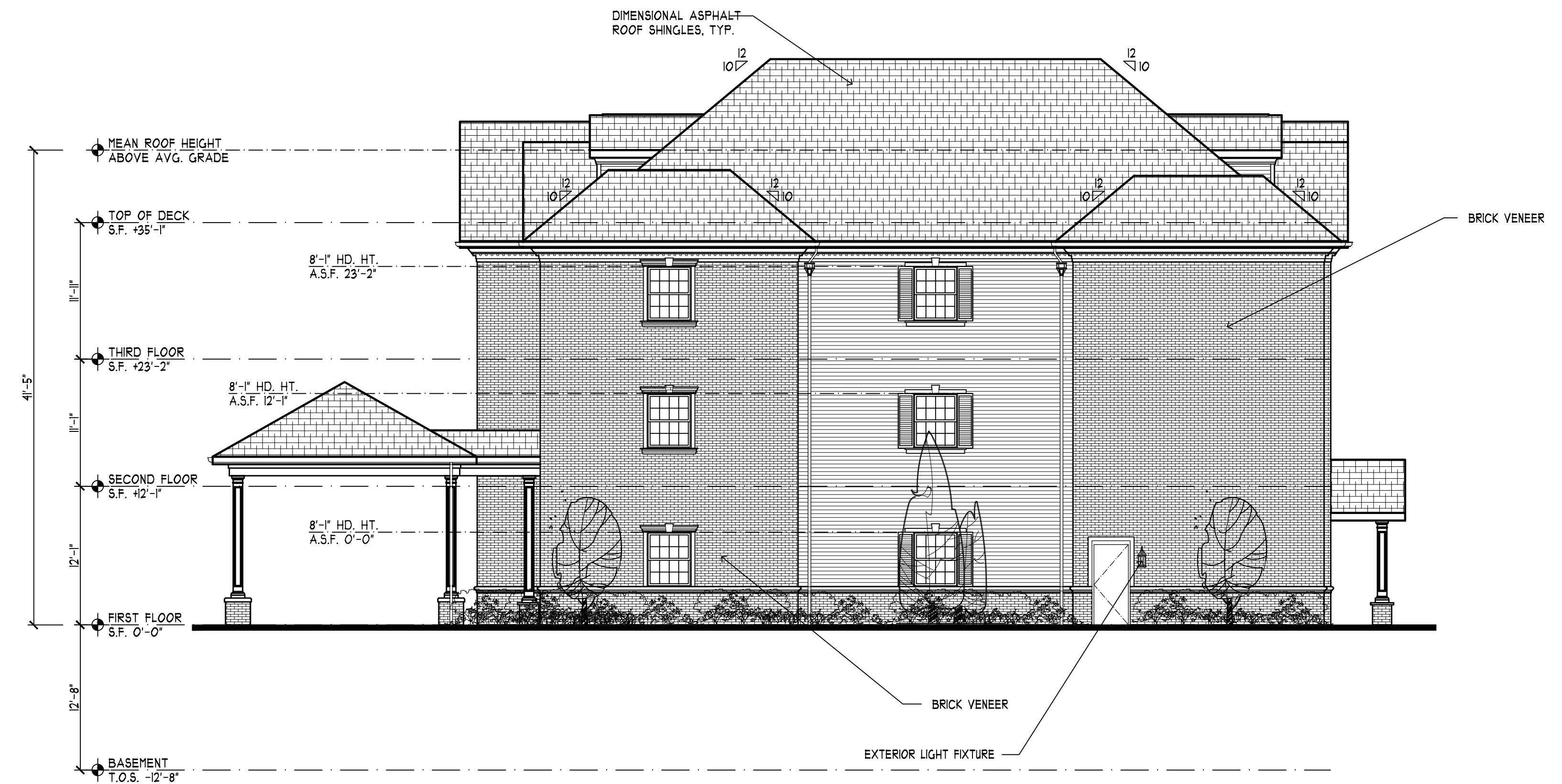
RIGHT SIDE ELEVATION (SEE FRONT ELEVATION FOR TYPICAL MATERIALS) SCALE: 1/8" = 1'-0"
