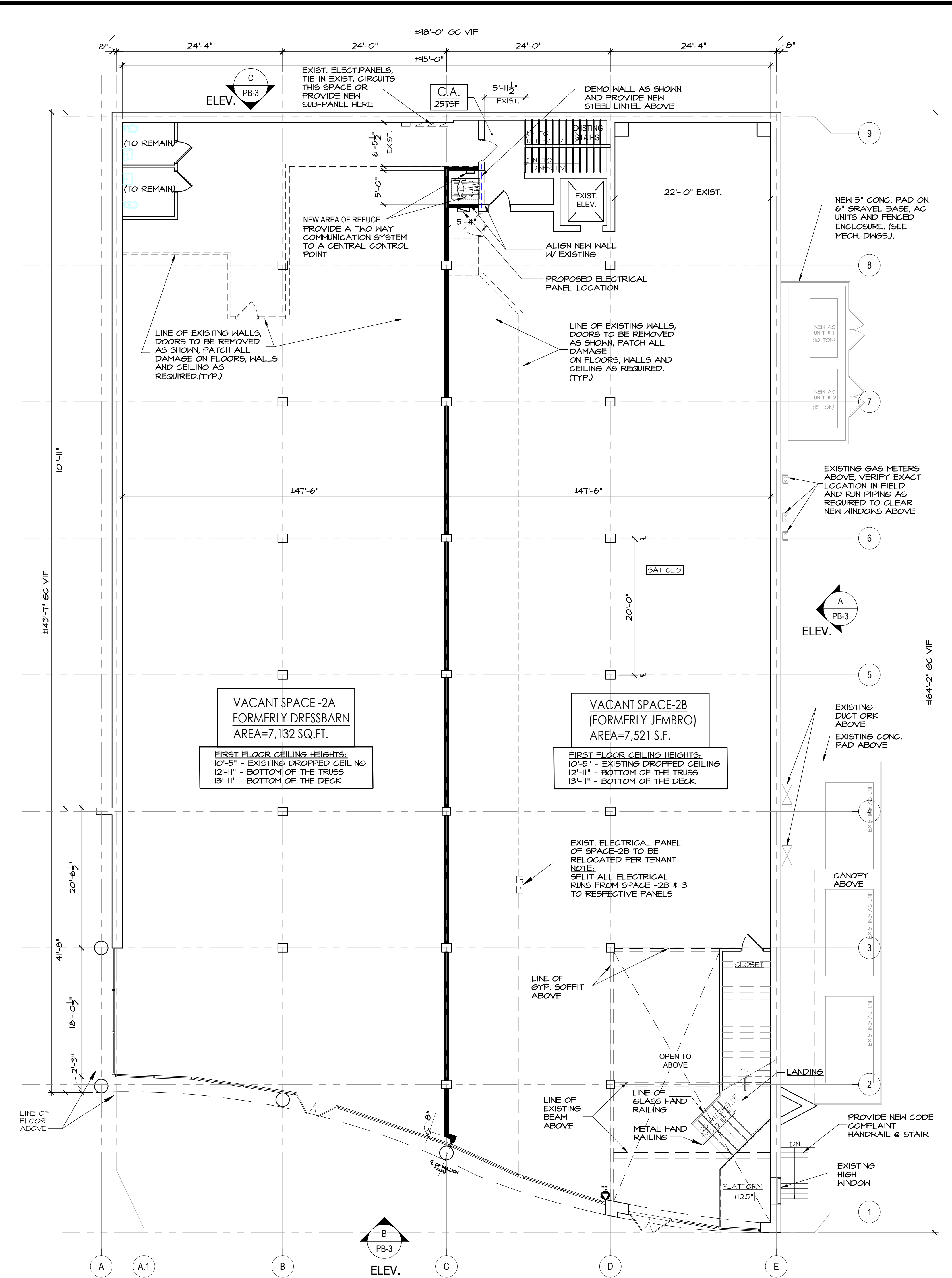
2 2ND FLOOR DEMOLITION & PROPOSED PLAN SCALE: 1/8" = 1'-0"
