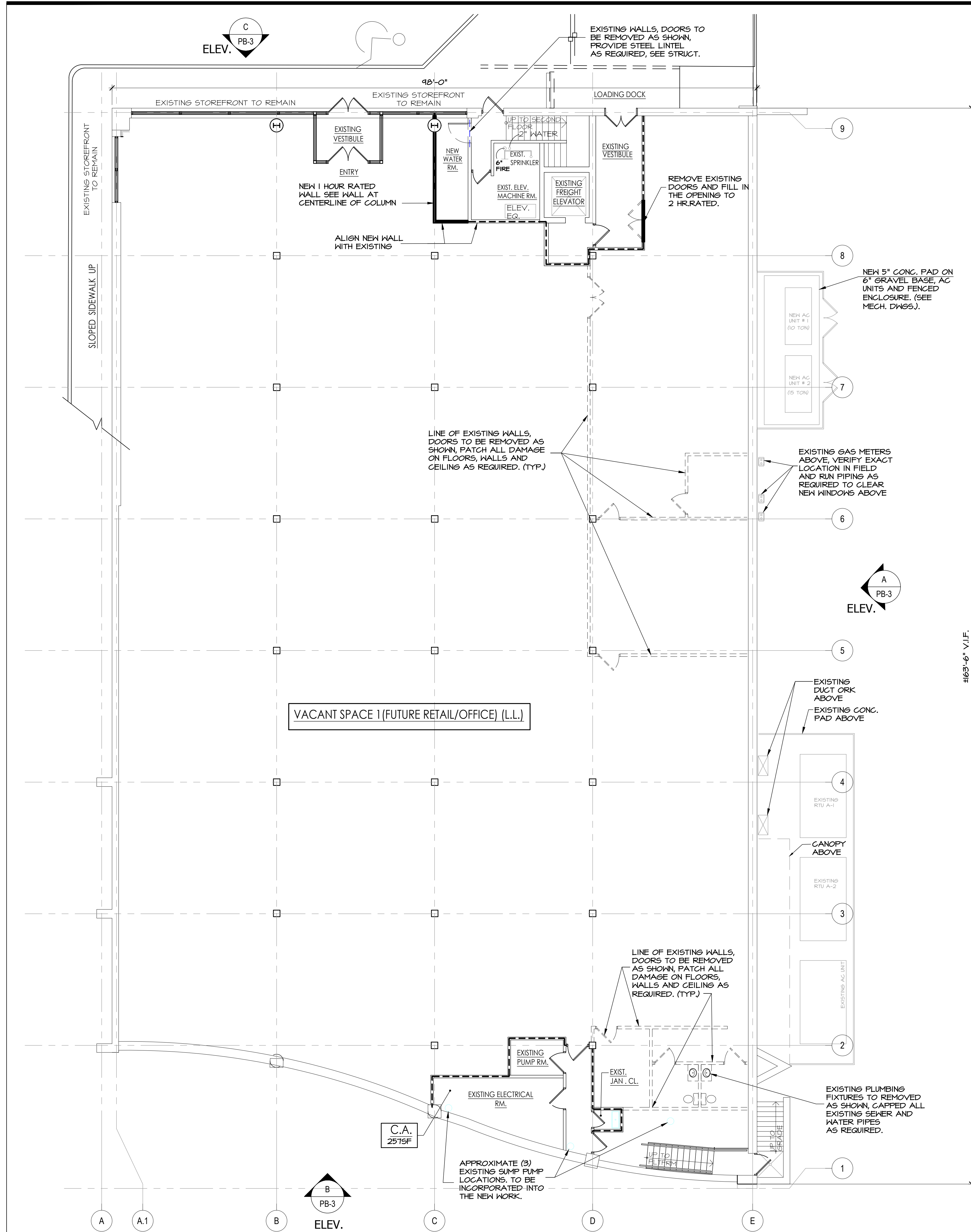
1 1ST FLOOR DEMOLITION & PROPOSED PLAN SCALE: 1/8" = 1'-0"
